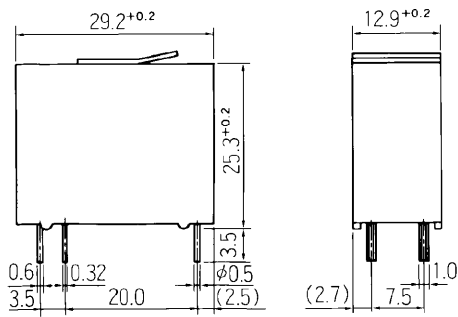
VS-C type (Plastic sealed type with tape)
