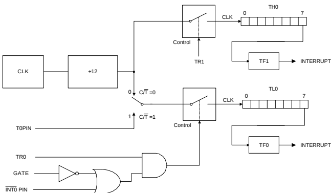
FIGURE 13: TIMER/COUNTER 0 MODE 3
