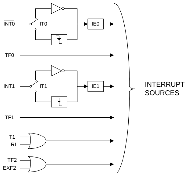
FIGURE 21: INTERRUPT SOURCES
