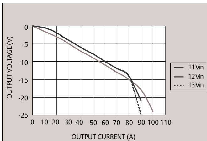
Figure 2: Load Regulation
