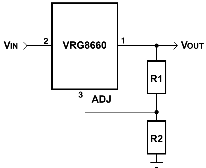
Adjustable Regulator
