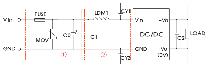
12VDC nominal input series
