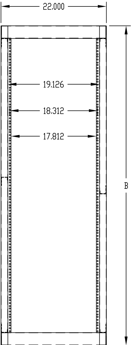
FRONT VIEW
