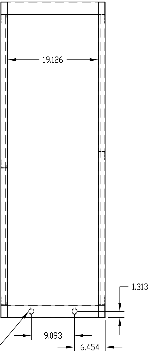
REAR VIEW
