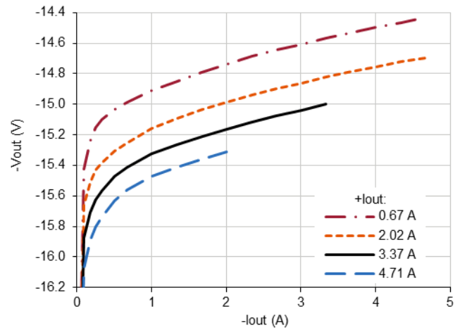
4.2.2 VPT100+2815D -V out (V) vs. -I out (A)
