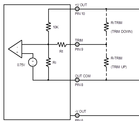
Output Voltage Trim Circuit
