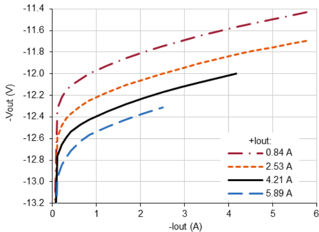
4.2.1 VPT100+2812D -V out (V) vs. -I out (A)
