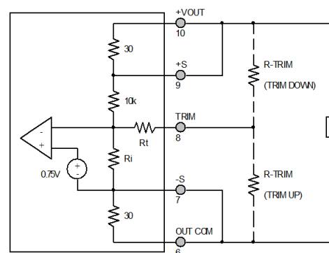
Output Voltage Trim Circuit
