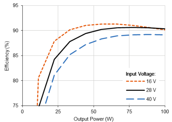
4.1.4 VPT100+2812S Efficiency (%) vs. Output Power (W)
