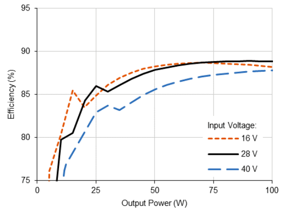
4.1.6 VPT100+2828S Efficiency (%) vs. Output Power (W)
