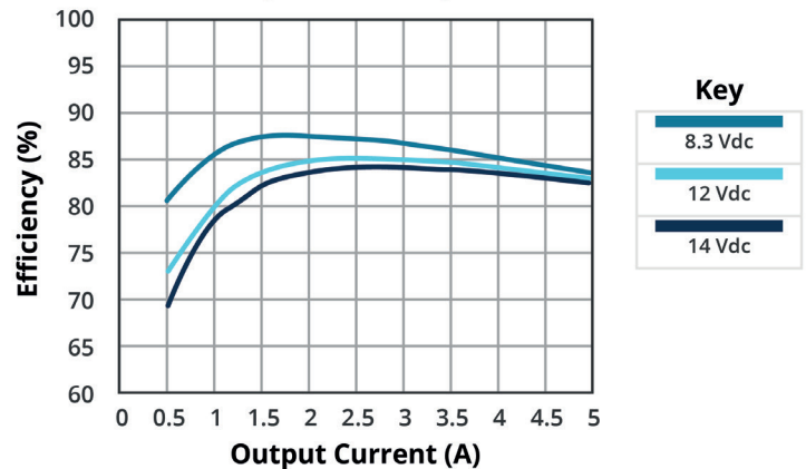
EFFICIENCY VS OUTPUT CURRENT VPOL5A-12-SMT ( V_o = 0.75 Vdc)
