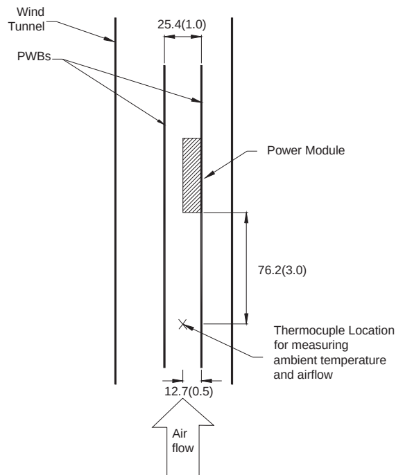
Figure 10. Temperature Measurement Location for VPOL20A-12W-SMT
