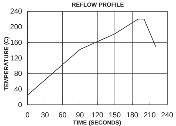
Figure 17 VPOL20A-12W-SMT Reflow Profile
