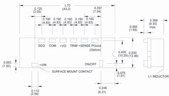
Figure 18 VPOL20A-12W-SMT Mechanical Outline Diagram
