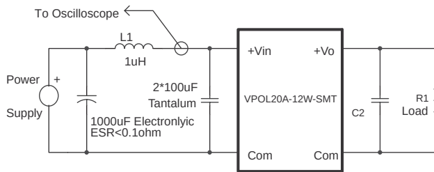
Figure 12. Input Reflected-Ripple Test Setup
