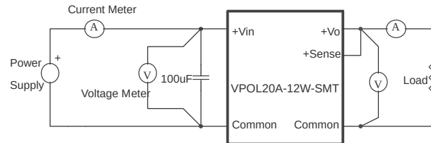
Figure 13. VPOL20A-12W-SMT Series Test Setup
