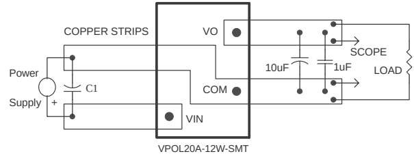
Figure 16. Output Voltage Ripple and Noise Measurement Set-Up
