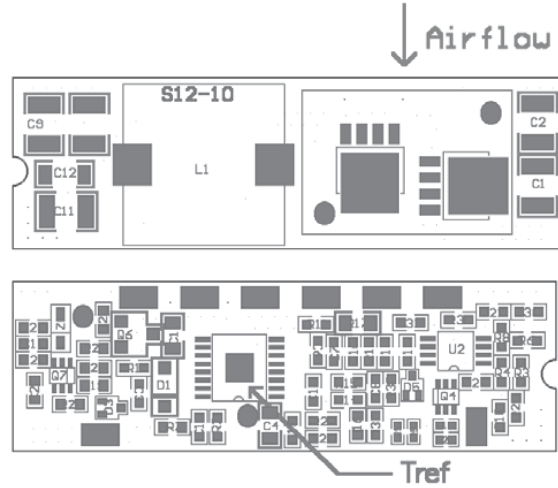
Figure 10. Temperature Measurement Location for VPOL20A-12W-SMT
