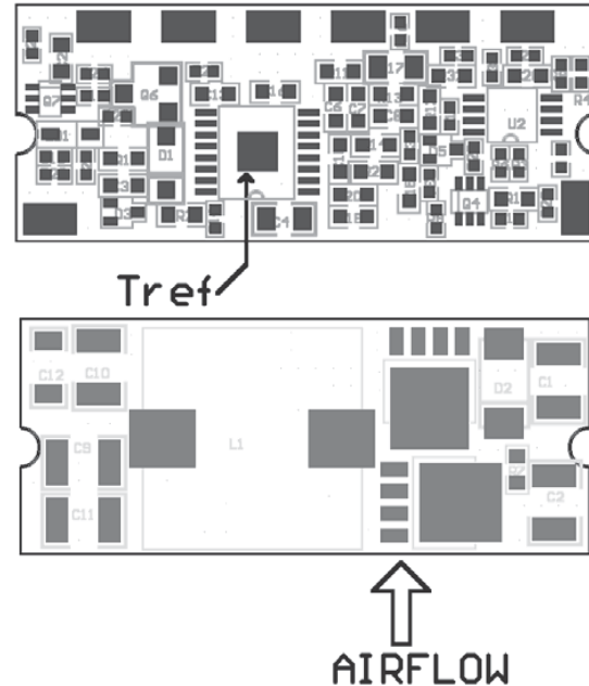
Figure 10. Temperature Measurement Location for VPOL10A-12W-SMT
