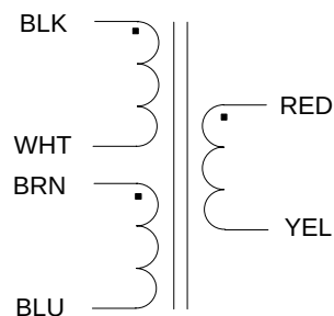
SCHEMATIC
