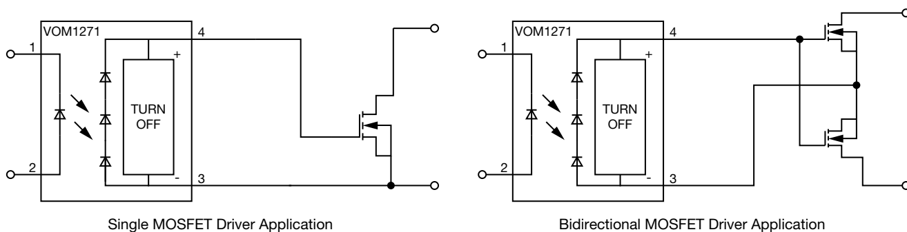
Fig. 10 - Typical Bidirectional MOSFET Driver Application with Integrated Fast Turn-Off
