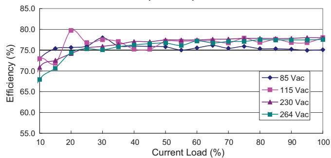
5 Vdc Output Efficiency Curve (at 25°C)
