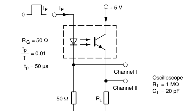
Fig. 2 - Test Circuit, Non-Saturated Operation
