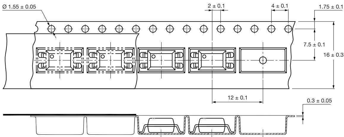
Fig. 18 - Tape and Packing for Option 7 (1000 units per reel)
