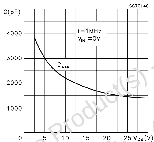
Figure 11. Capacitance Variations
