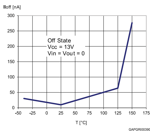
Figure 15: OFF-state output current
