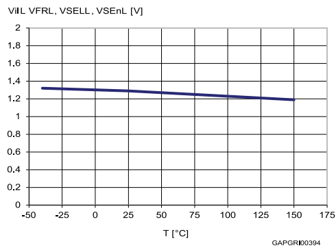
Figure 19: Logic Input low level voltage
