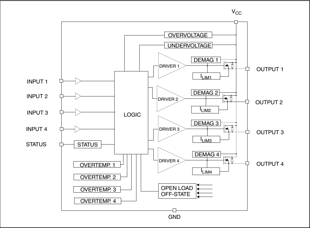
Figure 1. Block diagram
