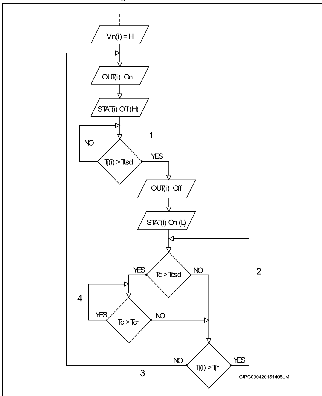
Figure 14: Thermal behavior
