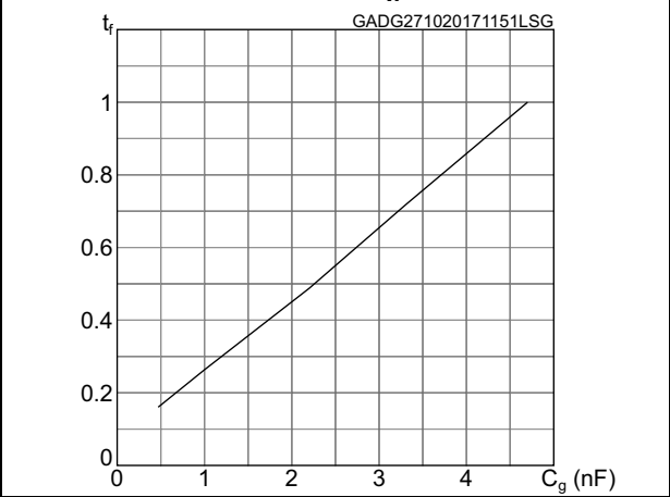
Figure 15. Gate driver low side fall time normalized vs C q = 4.7nF
