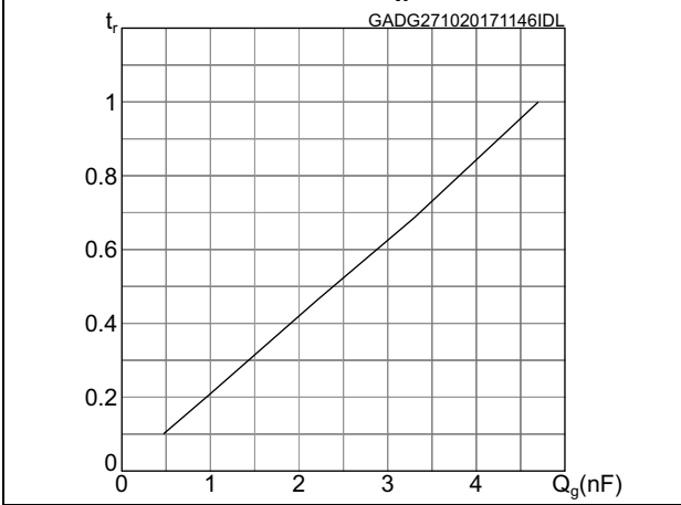
Figure 14. Gate driver low side rise time normalized vs C q = 4.7nF
