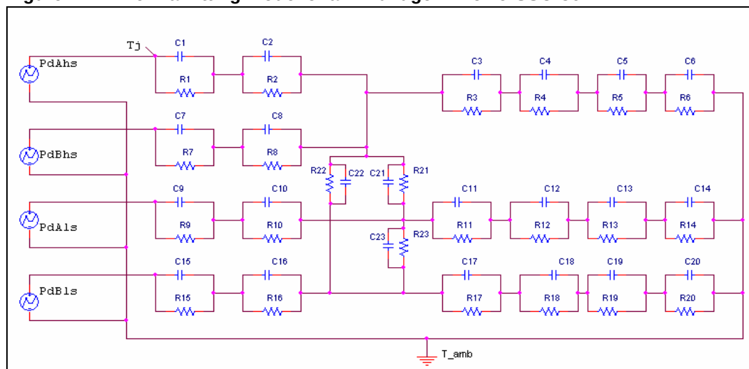
Figure 21. Thermal fitting model of an H-bridge in PowerSSO-36
