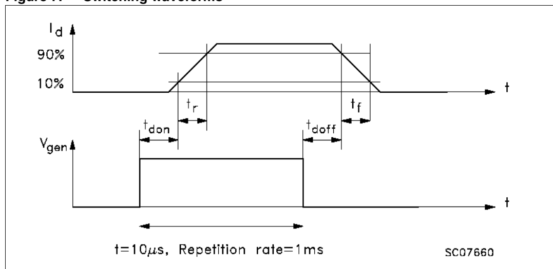
Figure 7. Switching waveforms
