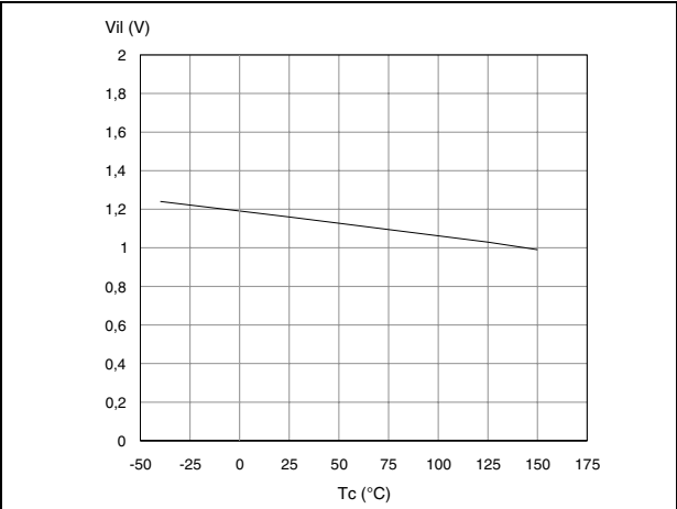
Figure 20. Input low level (Vil) vs. temperature (Tc). The graph shows Vil (V) on the y-axis (0 to 2) and Tc (°C) on the x-axis (-50 to 175). The curve decreases linearly from approximately 1.25 V at -50°C to 1.0 V at 150°C.
