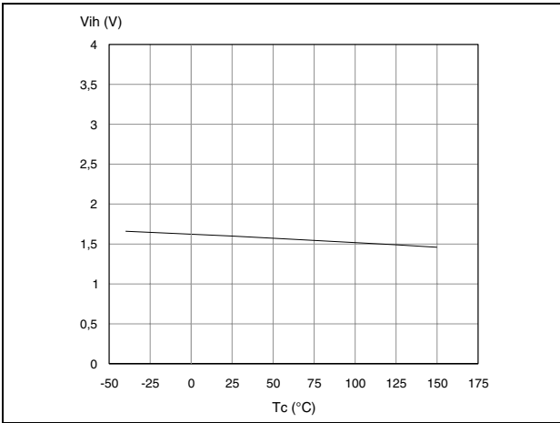
Figure 21. Input high level (Vih) vs. temperature (Tc). The graph shows Vih (V) on the y-axis (0 to 4) and Tc (°C) on the x-axis (-50 to 175). The curve decreases linearly from approximately 1.7 V at -50°C to 1.5 V at 150°C.
