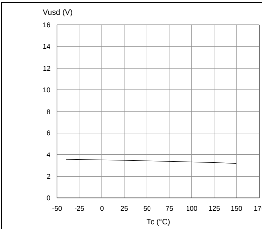
Figure 25. Undervoltage shutdown
