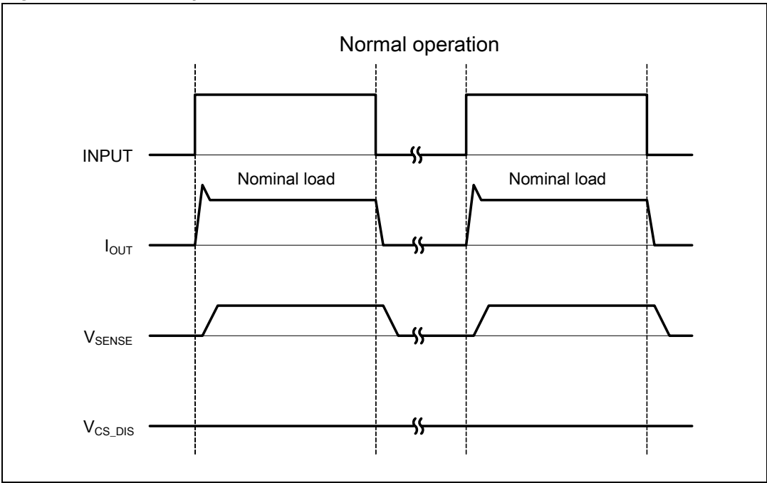
Figure 11. Normal operation
