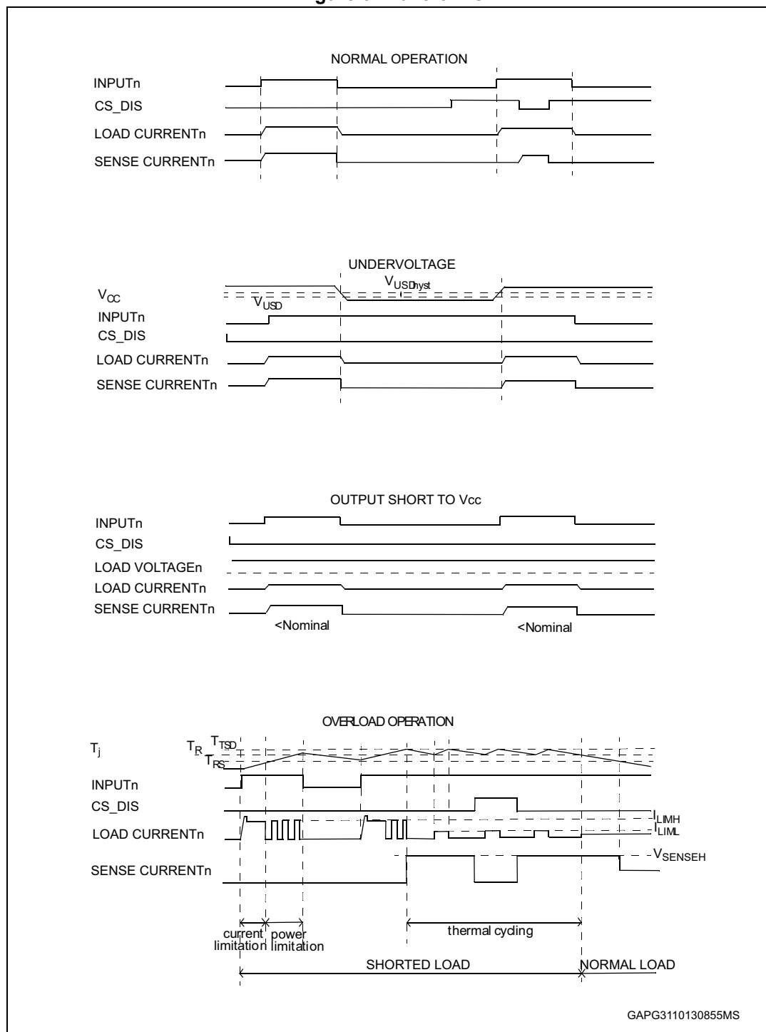
Figure 6. Waveforms
