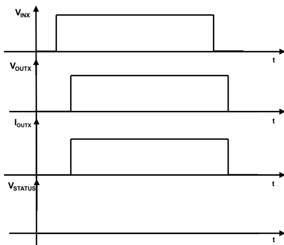
Figure 6. Switching on resistive load
