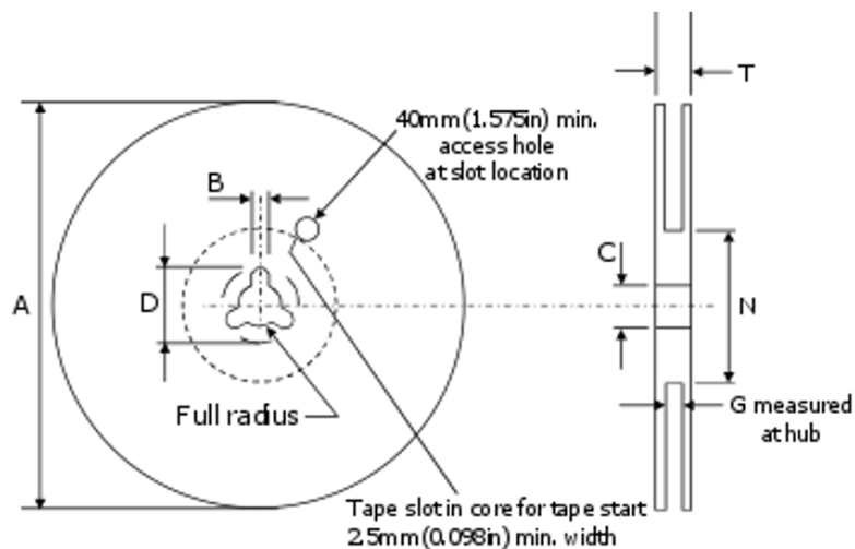
Figure 21. Reel specifications
