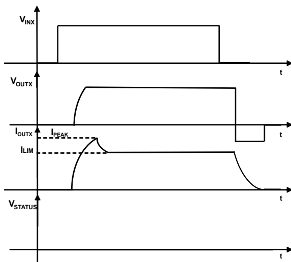
Figure 9. Switching on heavy inductive load
