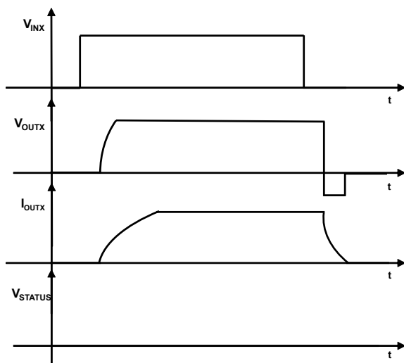
Figure 8. Switching on light inductive load
