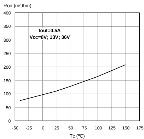
Figure 14. On State Resistance Vs T case
