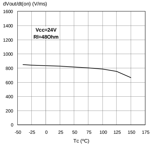
Figure 18. Turn-on Voltage Slope
