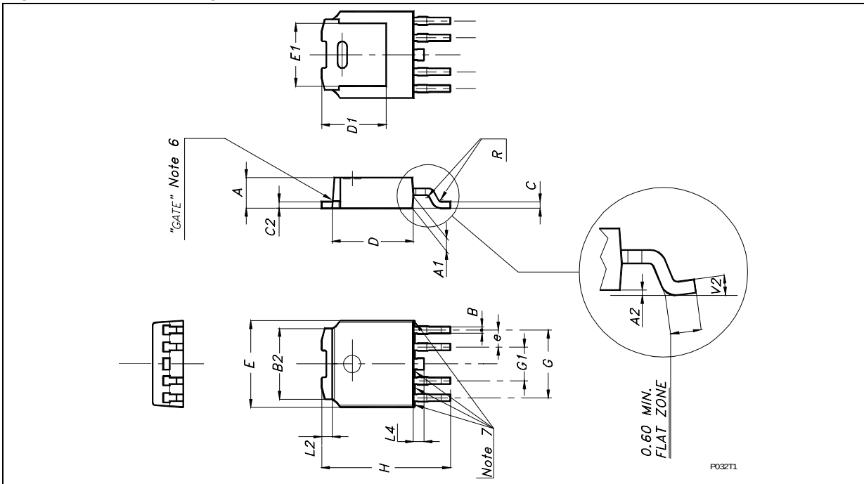
Figure 34. PPAK Package Dimensions
