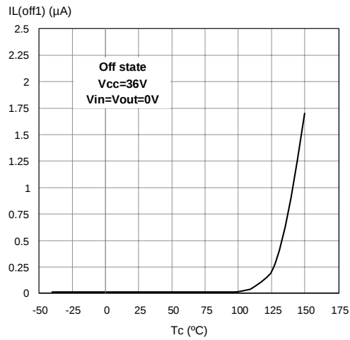
Figure 11. Off State Output Current
