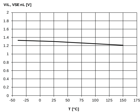
Figure 12: Logic Input low level voltage
