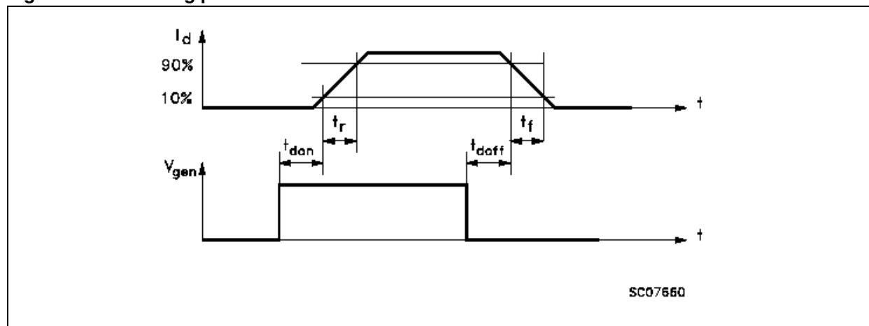
Figure 8. Switching parameter test conditions
