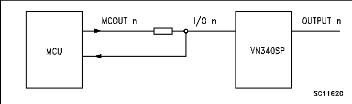
Figure 9. Driving circuit
