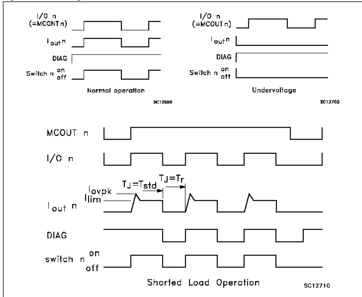
Figure 7. Switching waveforms
