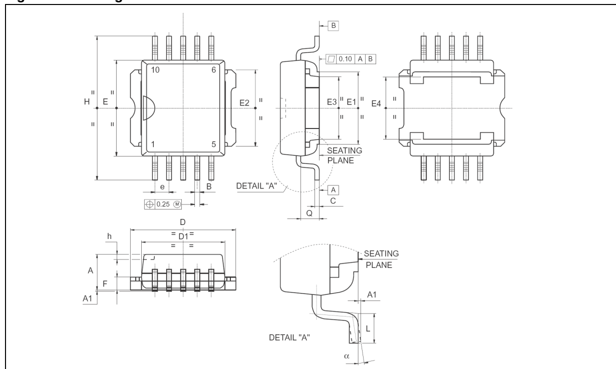
Figure 10. Package dimension
