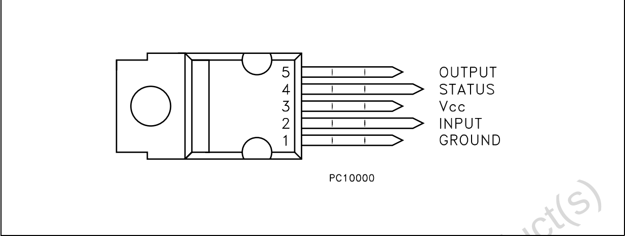
Figure 3. Connection Diagram
