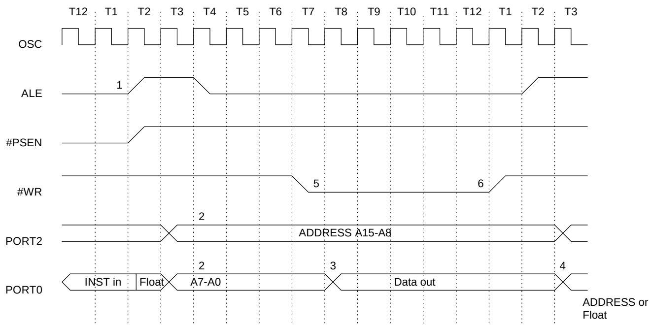
FIGURE 27: DATA MEMORY WRITE CYCLE TIMING
