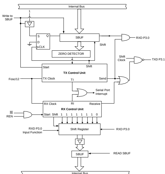
FIGURE 12: SERIAL PORT MODE 0 BLOCK DIAGRAM
