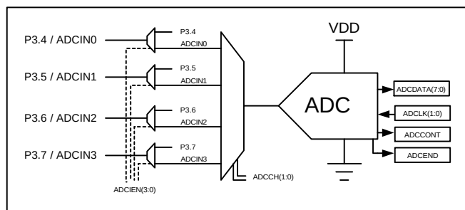
FIGURE 18: ADC STRUCTURE
