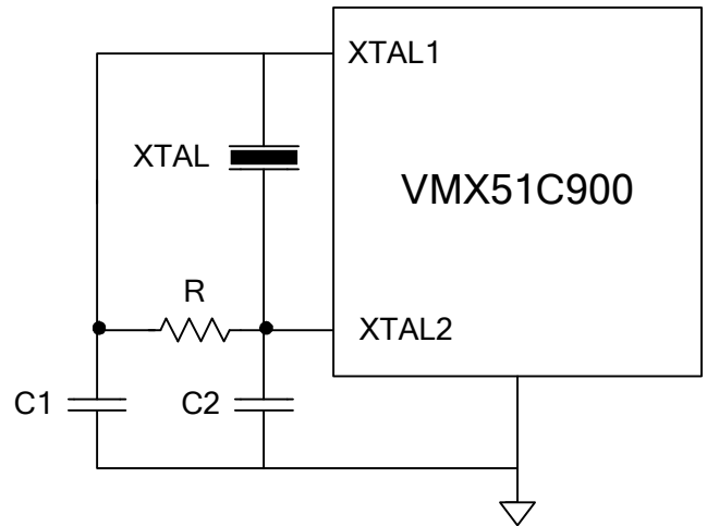
FIGURE 22: CRYSTAL CONFIGURATION
