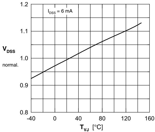
Fig. 1 Drain source breakdown voltage V_{DS} versus junction temperature T_{VJ}
