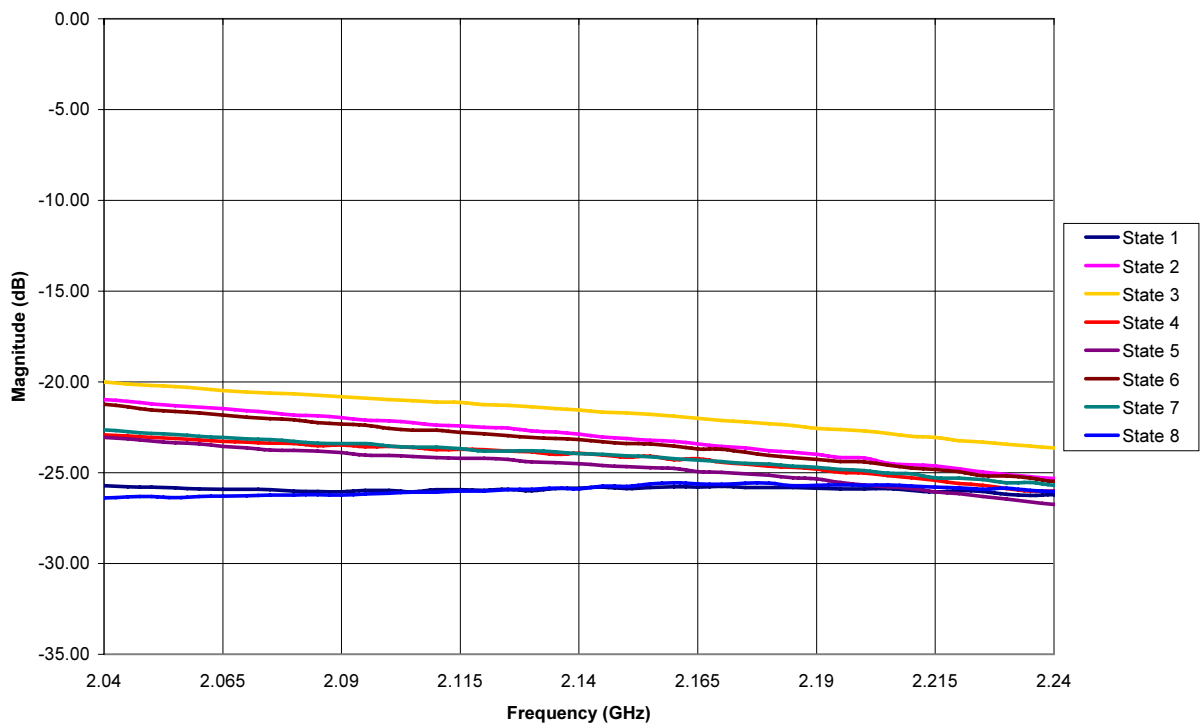
Input Return Loss, 8-States
