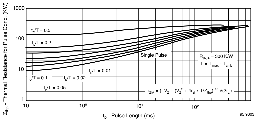
Fig. 10 - Thermal Response
