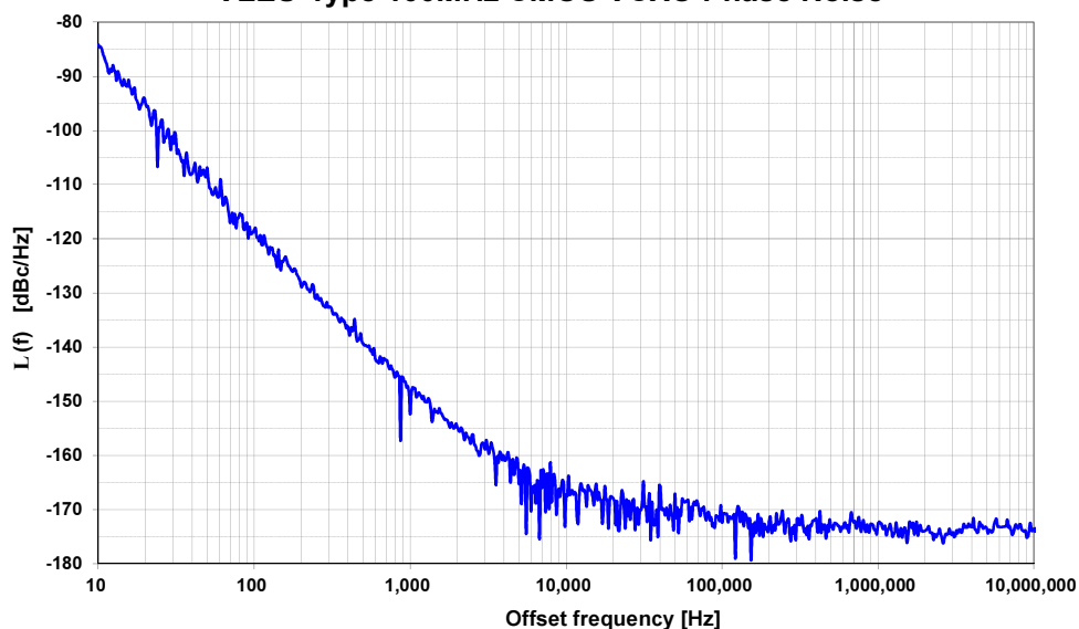
VLEU-Type 100MHz CMOS VCXO Phase Noise
