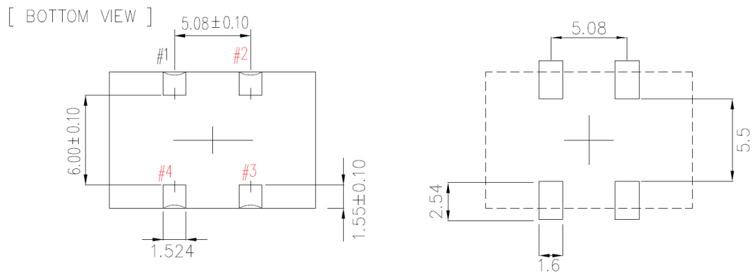
Recommended Soldering Pattern
