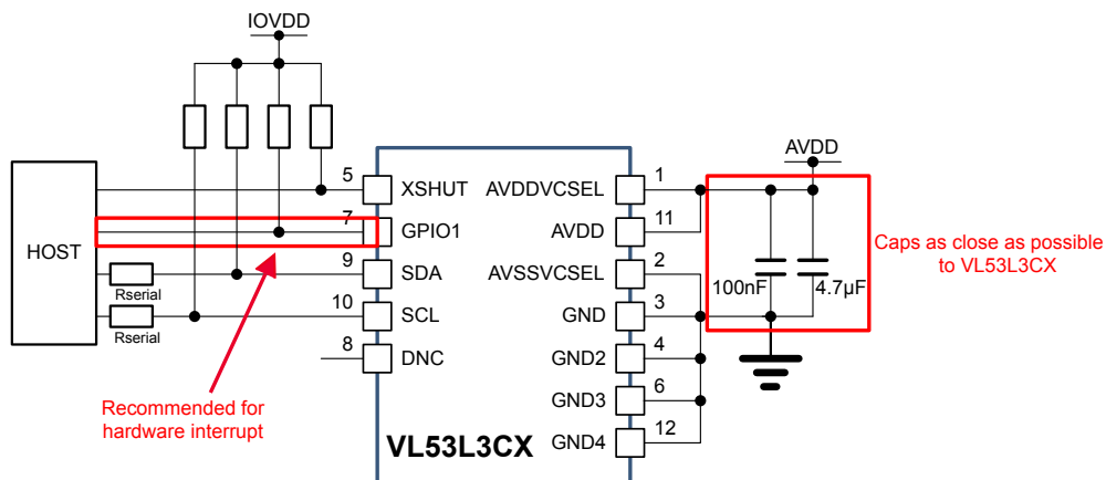
Figure 3. VL53L3CX schematic
