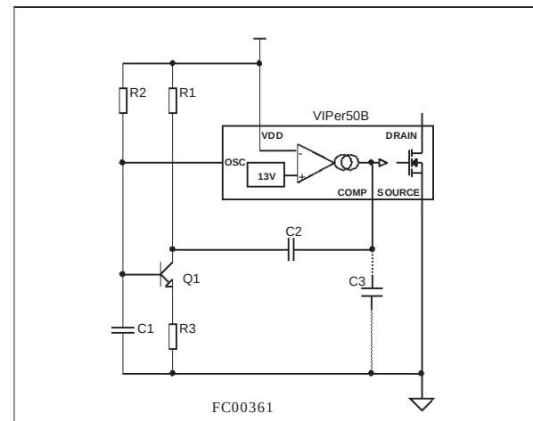
Figure 19: Slope Compensation
