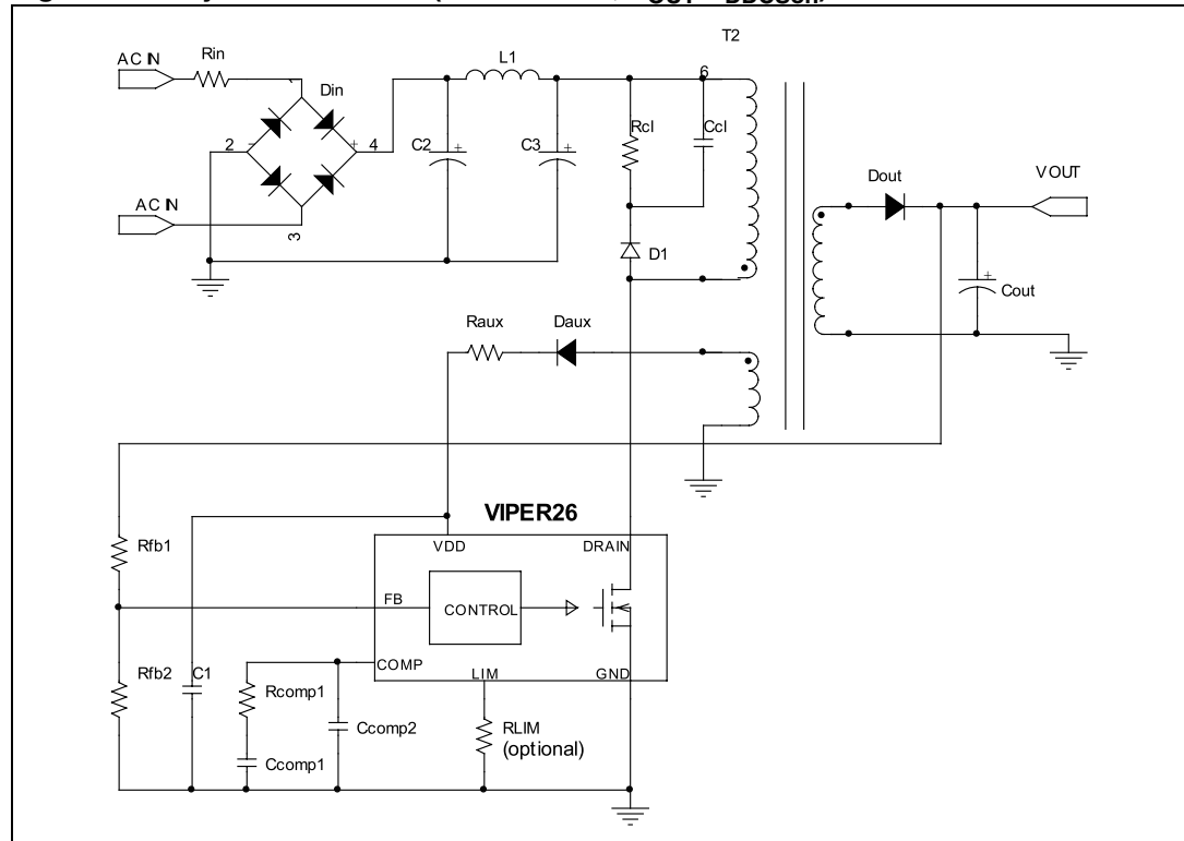
Figure 21. Flyback converter (non isolated, V_{OUT} \approx V_{DDCSon} )
