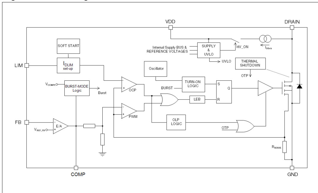
Figure 2. Block diagram
