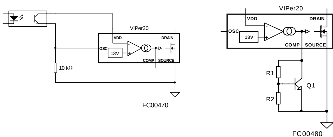
Figure 21. External Clock Synchronisation Figure 22. Current Limitation Circuit Example
