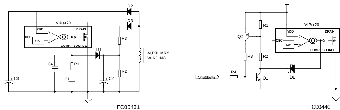
Figure 17. Mixed Soft Start and Compensation Figure 18. Latched Shut Down
