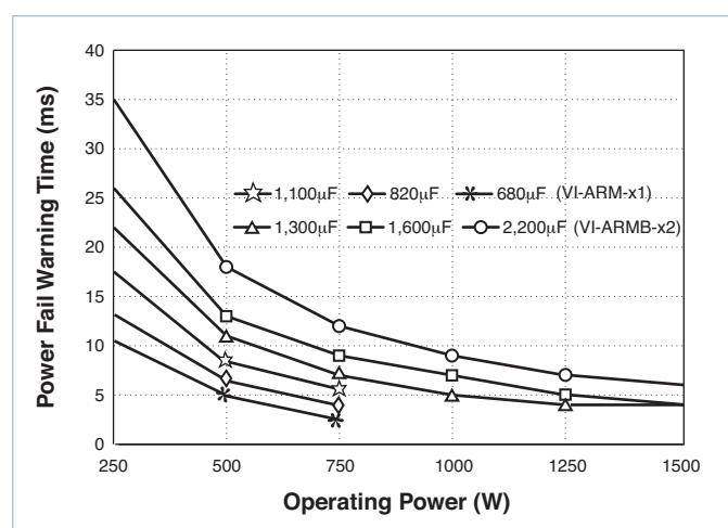
Figure 15 — Power fail warning time vs. operating power and total bus capacitance, series combination of C1, C2 (see Figure 10)
