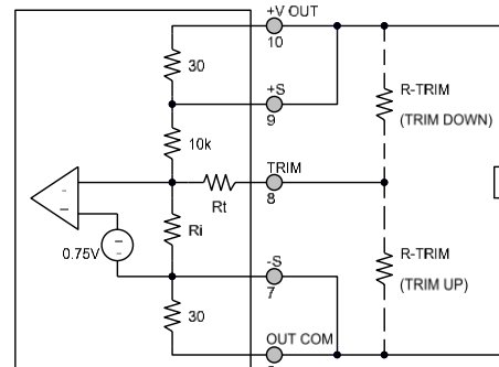
Output Voltage Trim Circuit
