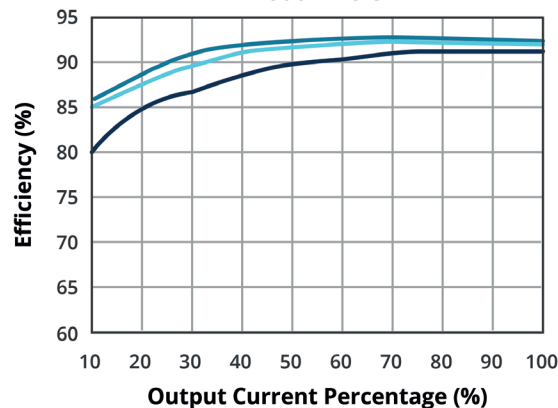
EFFICIENCY VS OUTPUT LOAD VFB600-D48-S24
