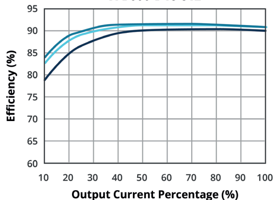
EFFICIENCY VS OUTPUT LOAD VFB600-D48-S12
