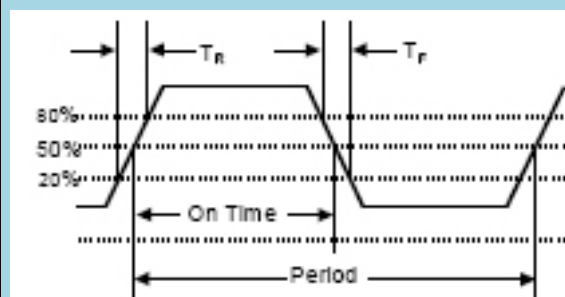
Output Waveform
