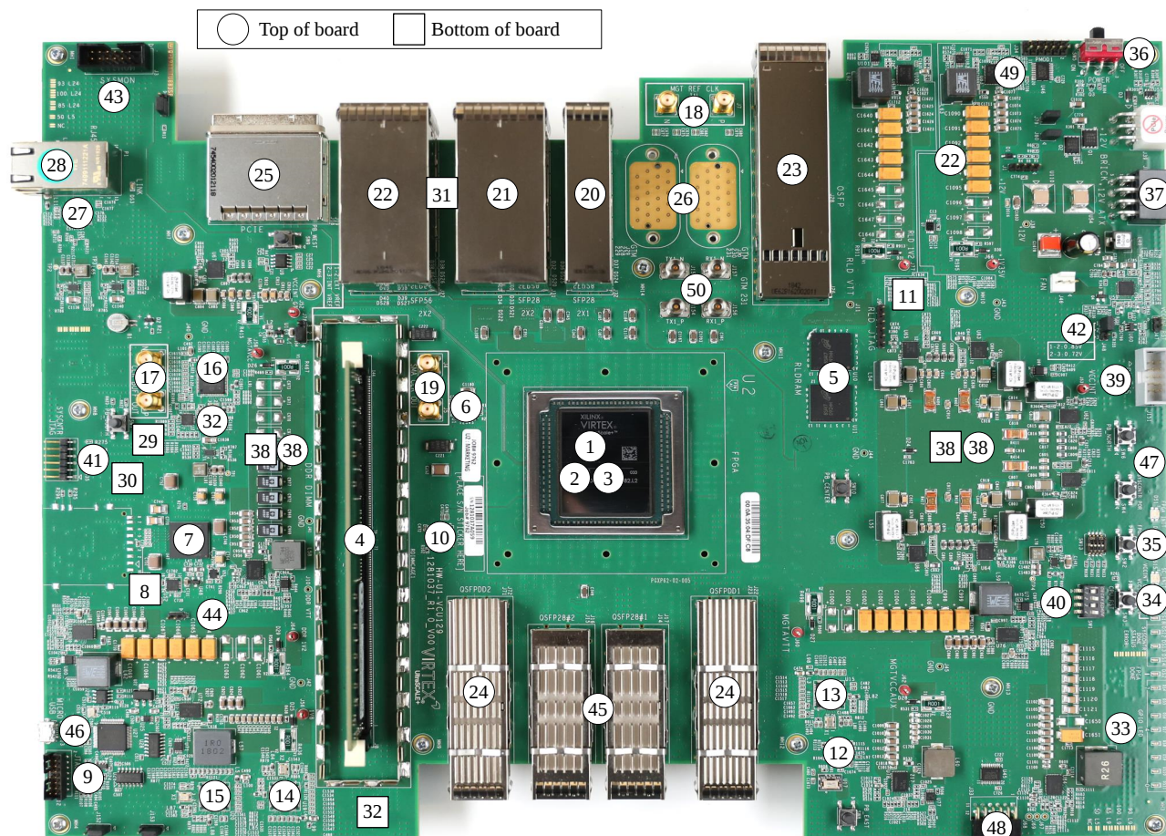
Figure 2: VCU129 Evaluation Board Component Locations
