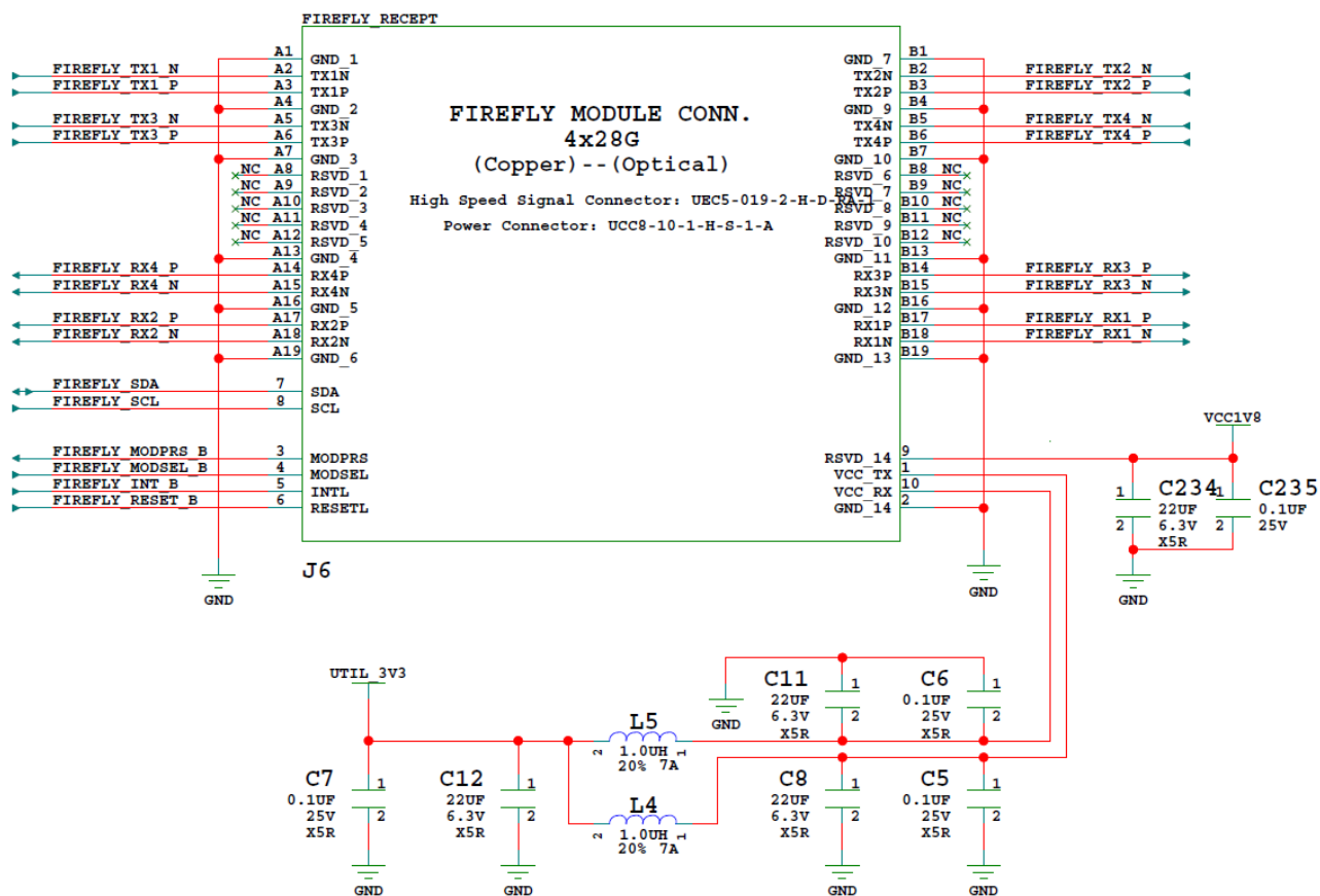
Figure 3-15: FireFly Connector Schematic
