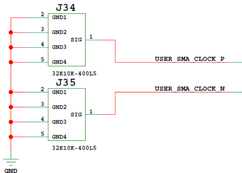
Figure 3-8: User SMA Clock
