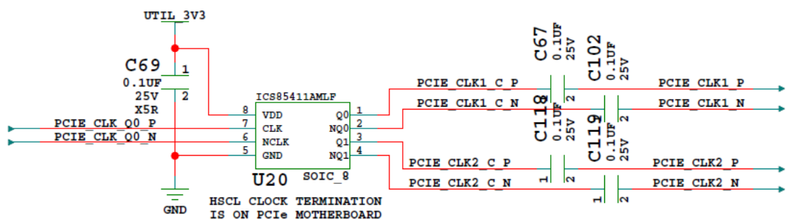
Figure 3-11: PCIe Clock
