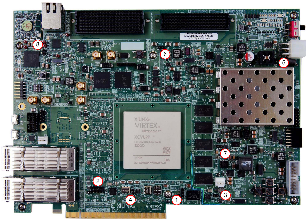
Figure 2-2: VCU118 Board Header Jumper Locations
