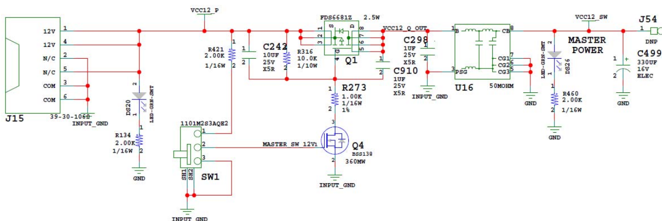
Figure 3-25: Power On/Off Switch SW1
