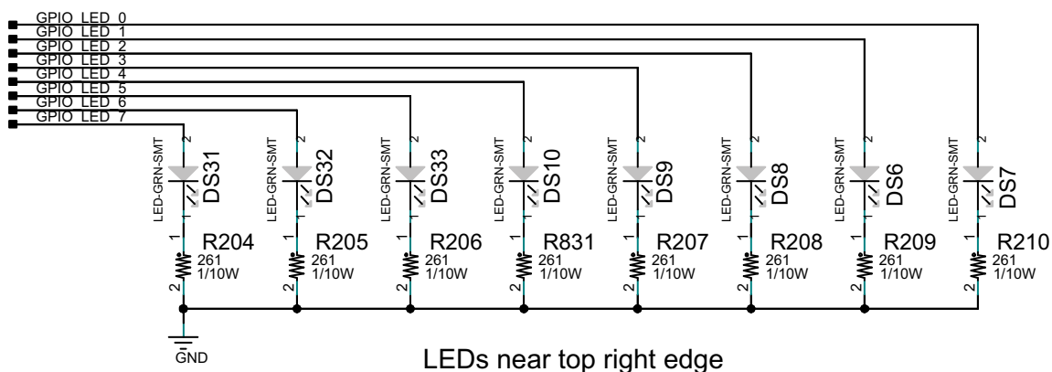
Figure 1-18: User LEDs
