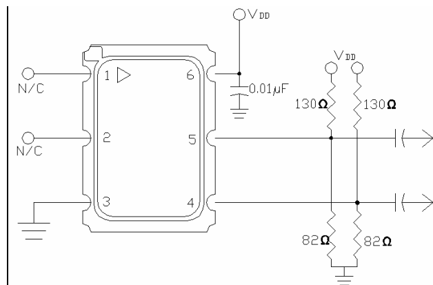
Figure 7. Pull-up Pull-down Termination
