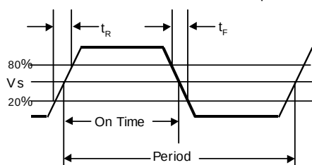
Figure 7. Output Waveform
