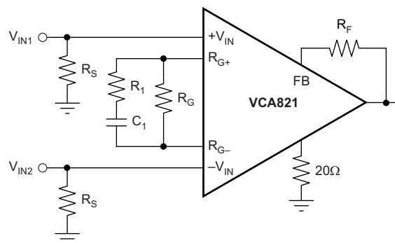
Figure 83. Differential Equalizer
